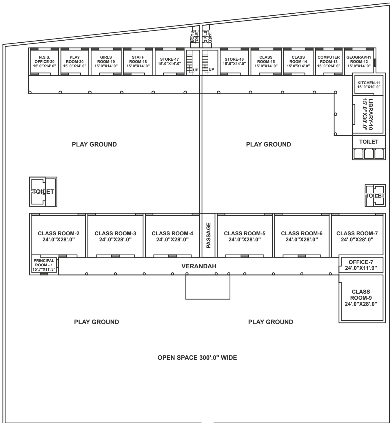
MAIN ROAD GROUND FLOOR PLAN
